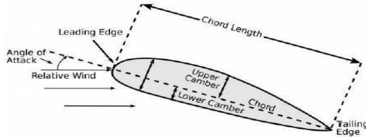
Fig: Basic Geometry of an Airfoil
