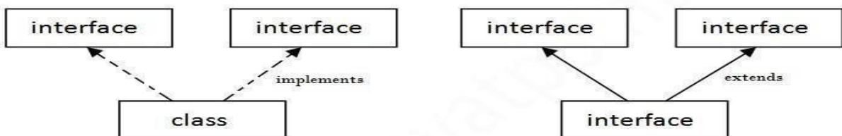
Multiple Inheritance in Java
