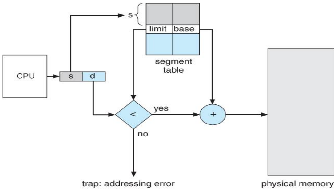
Figure 4.8 - Segmentation hardware
