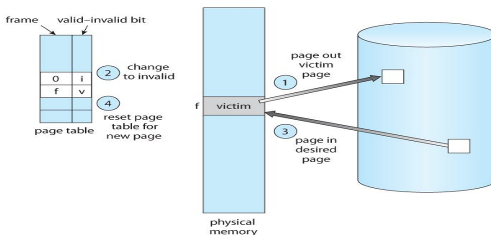
Figure 4.32 - Page replacement.
