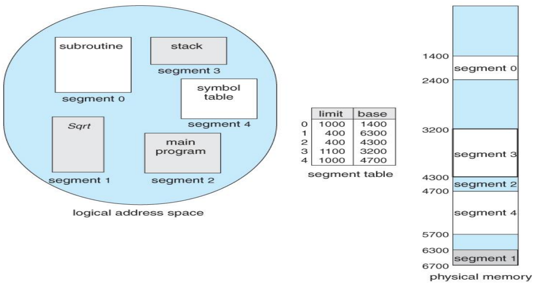
Figure 4.8 - Segmentation hardware
