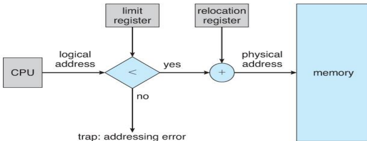
Figure 3.6 - Hardware support for relocation and limit registers
