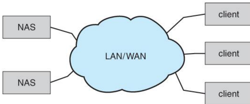
Figure 4.26- Network-attached storage.
