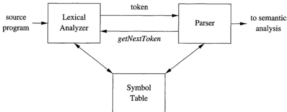
Figure 1.6 : Lexical Analyzer
