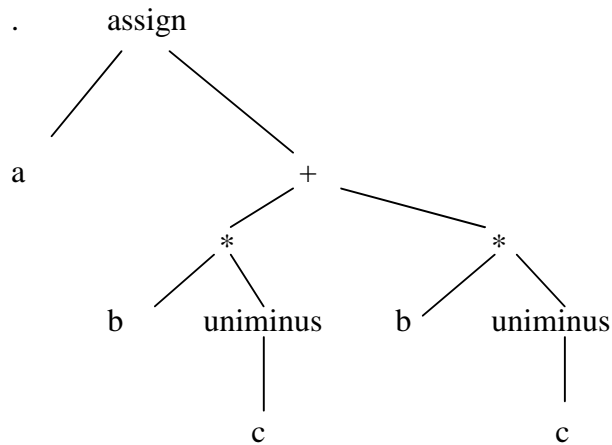
Figure 4.2 : Abstract Syntax Tree for the statement a:=b*-c+b*-c
