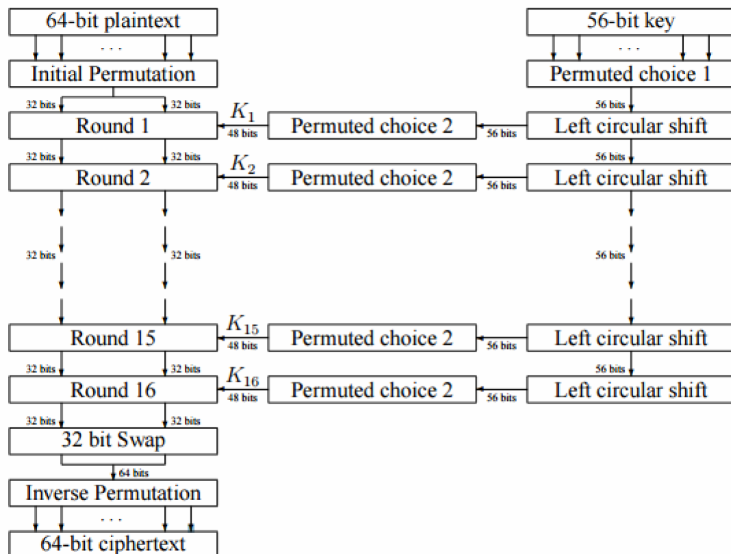
Figure : Flow Diagram of DES algorithm for encrypting data.
