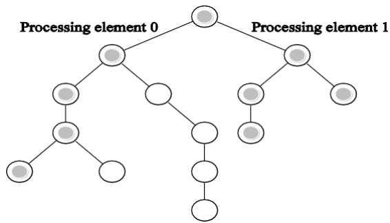
Searching an unstructured tree for a node with a given label, 'S', on two processing elements using depth-
