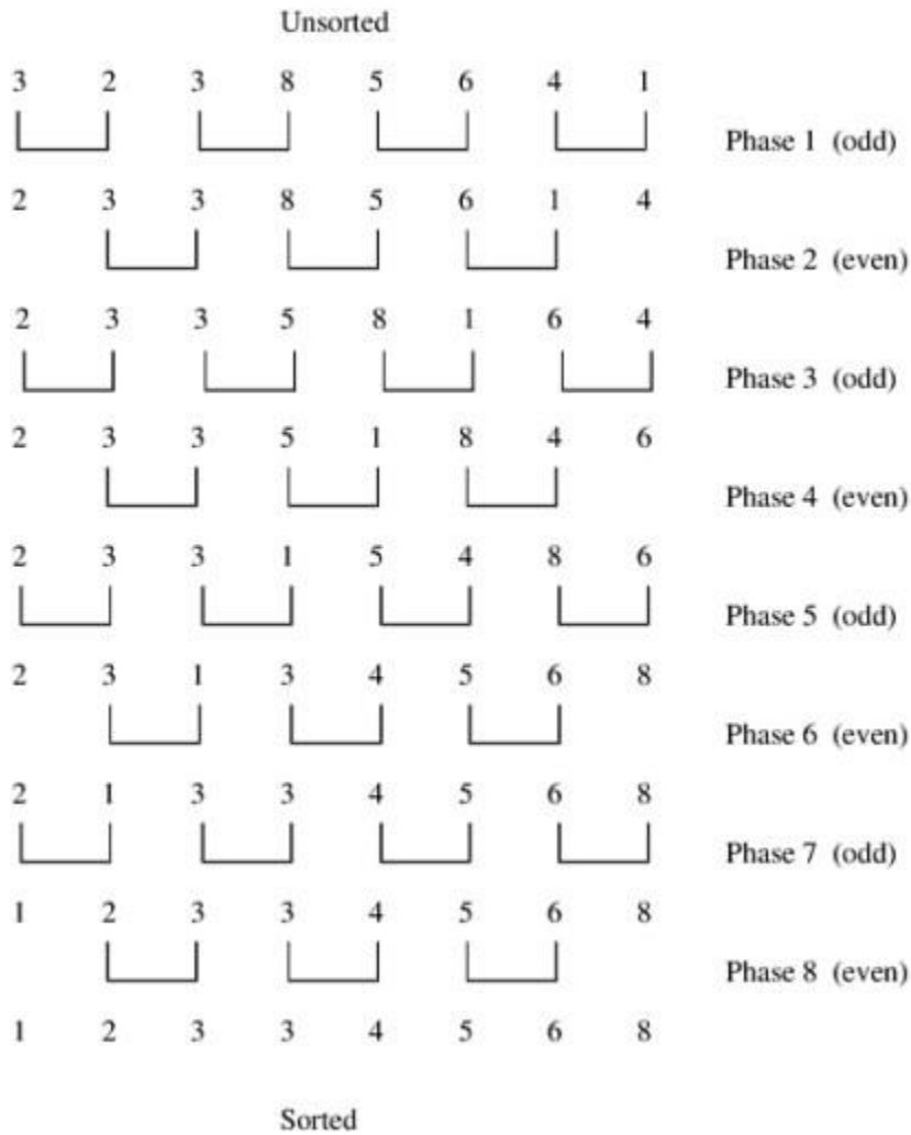
Algorithm 9.3 Sequential odd-even transposition sort algorithm.
