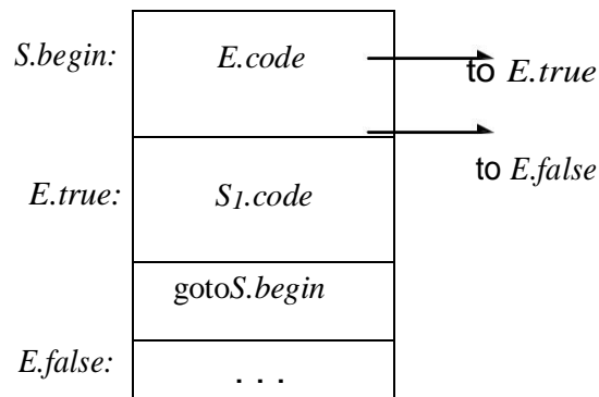
(c) while-do
