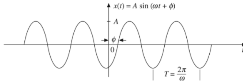
Figure 1.10 Sinusoidal waveform.
