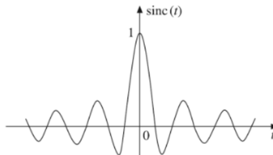
Figure 1.19 Sinc function.
