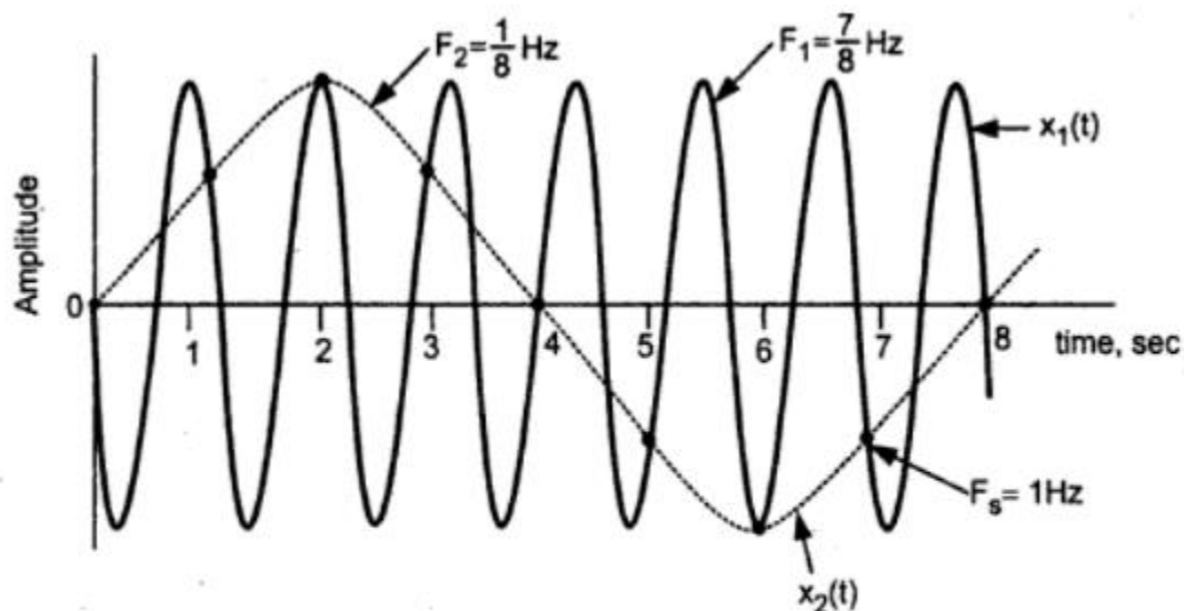
Fig. 5.1.5 Illustration of aliasing
