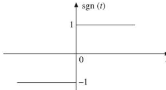
Figure 1.18 Signum function.
