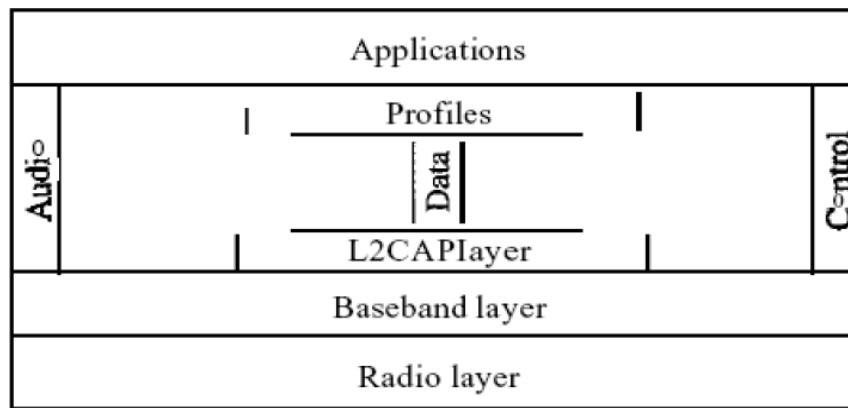
Figure 11 Bluetooth layers
