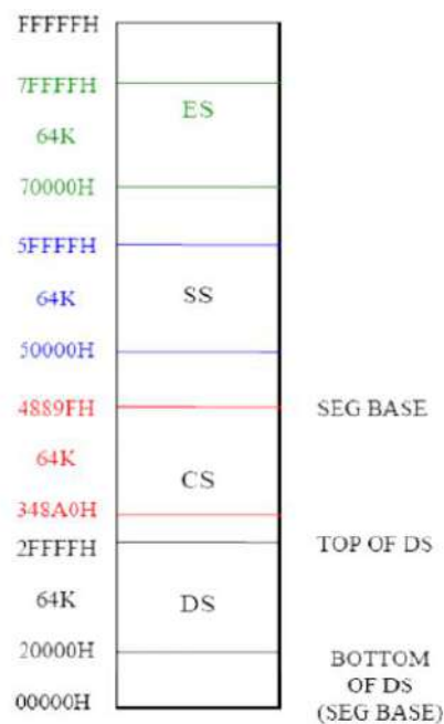
Fig1.5. Memory segmentation
