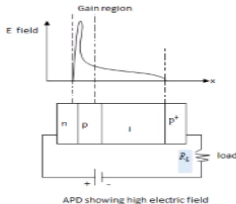
Figure 3.12: APD
