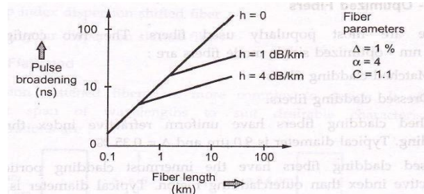
Fig. 2.8.1 Mode coupling effects on pulse broadening
