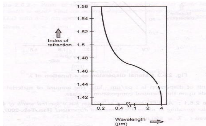
Fig. 2.6.2 Index of refraction as a function of wavelength
