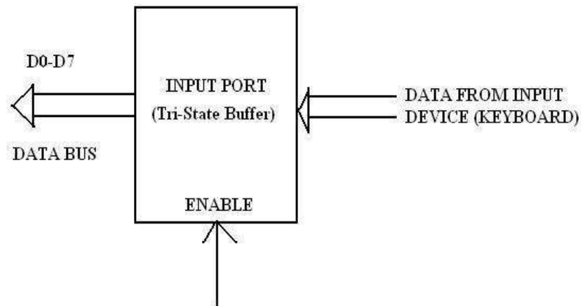
FIG.1 INPUT PORT
