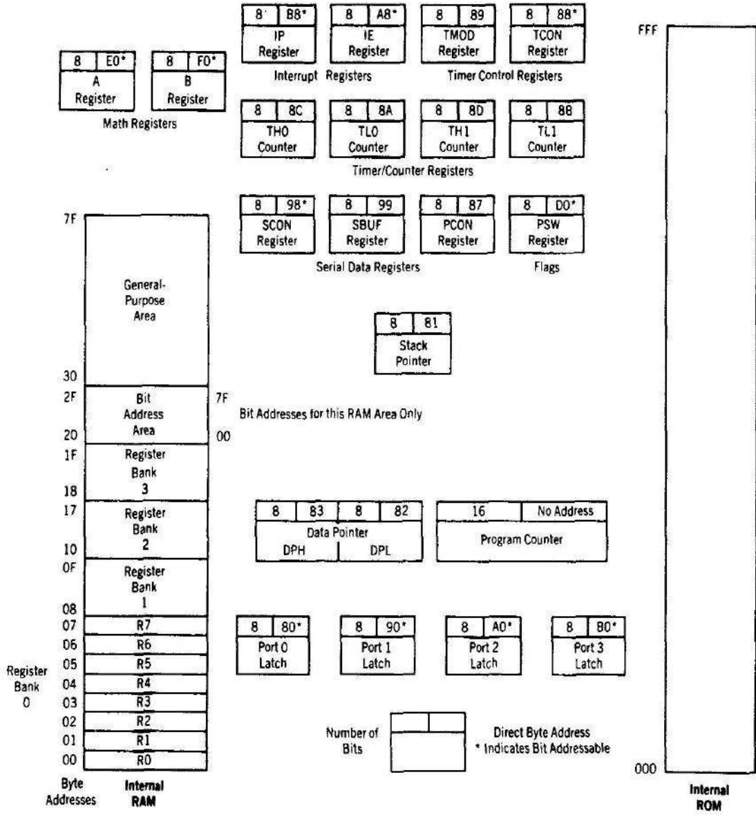
FIGURE 2.1b 8051 Programming Model
