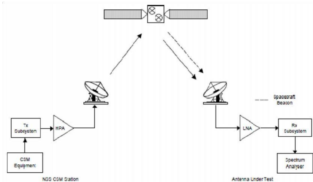
Figure 4.6 One possible arrangement for Measurement of G/T
