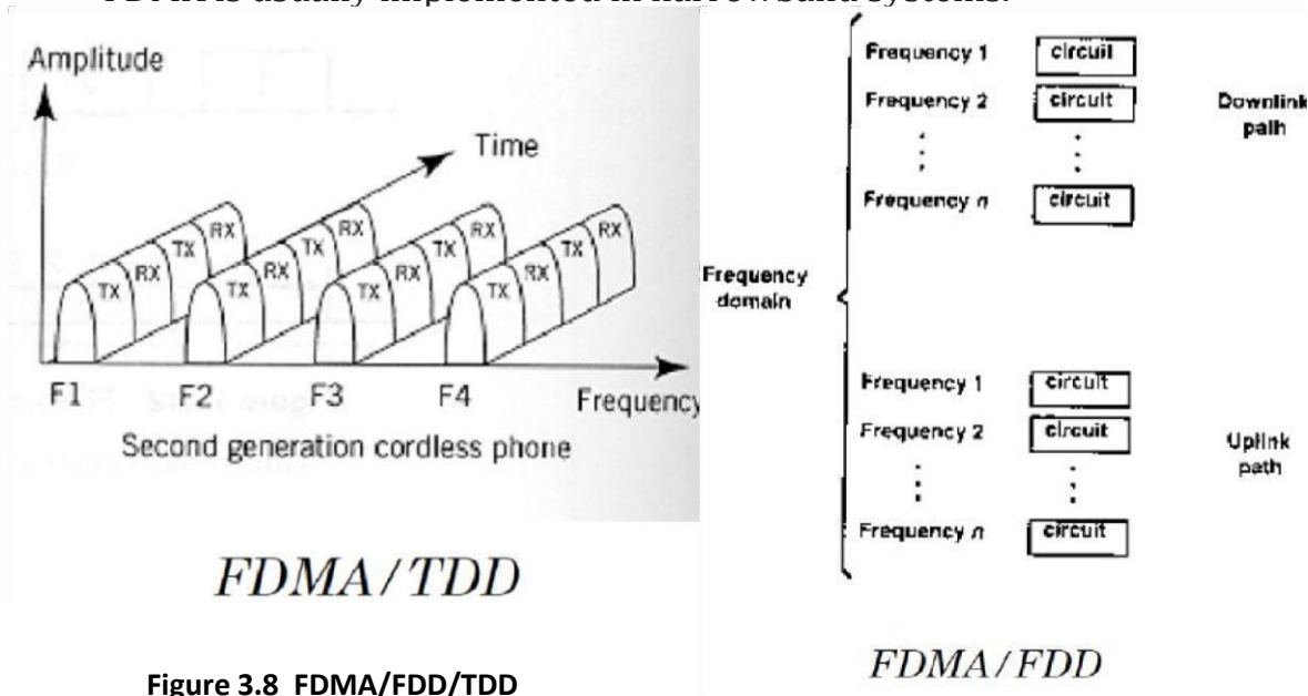
Figure 3.8 FDMA/FDD/TDD
