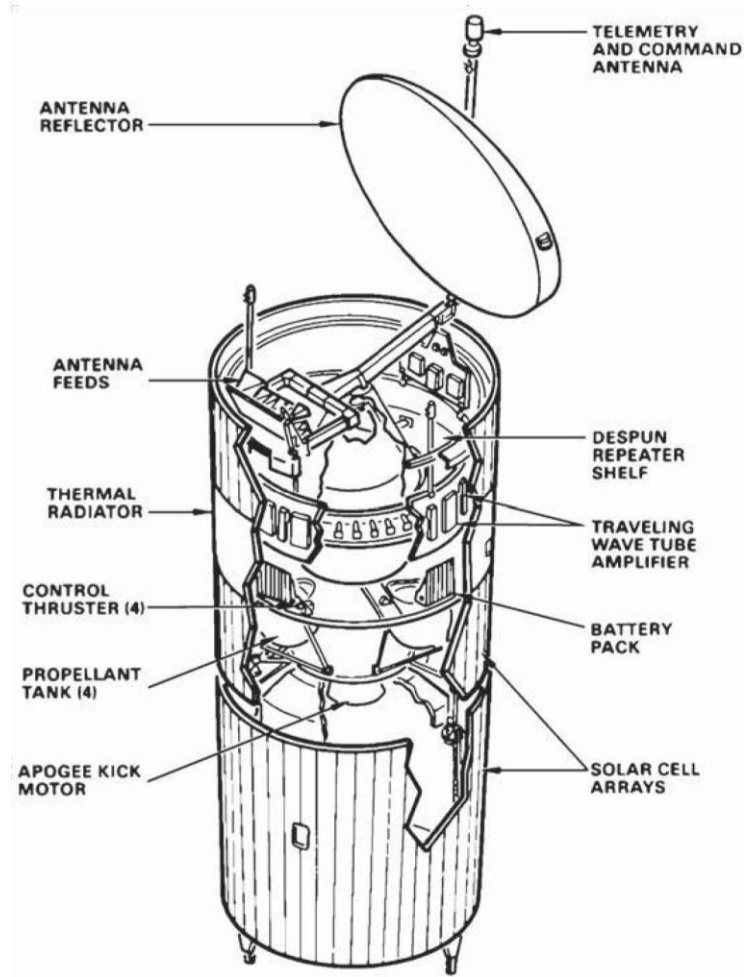
Figure 2.4 HS 376 spacecraft. (Courtesy of Hughes Aircraft Company Space and Communications Group.)
