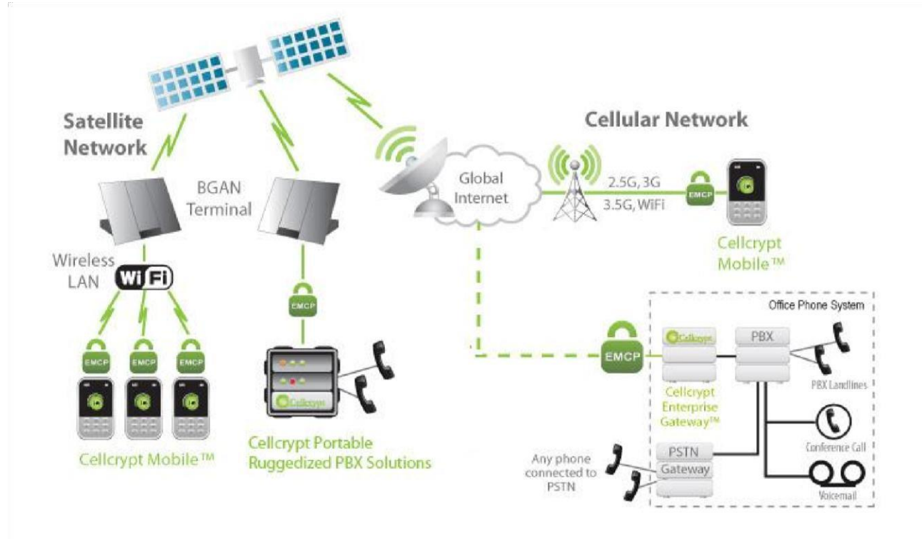
Figure 3.16 General block diagram Encryption methods
