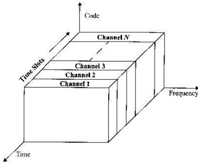
Figure 3.9 TDMA Channels
