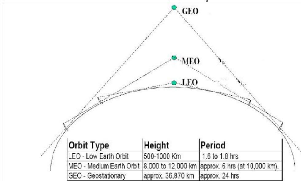
Figure 5.8 LEO, MEO & GEO range
