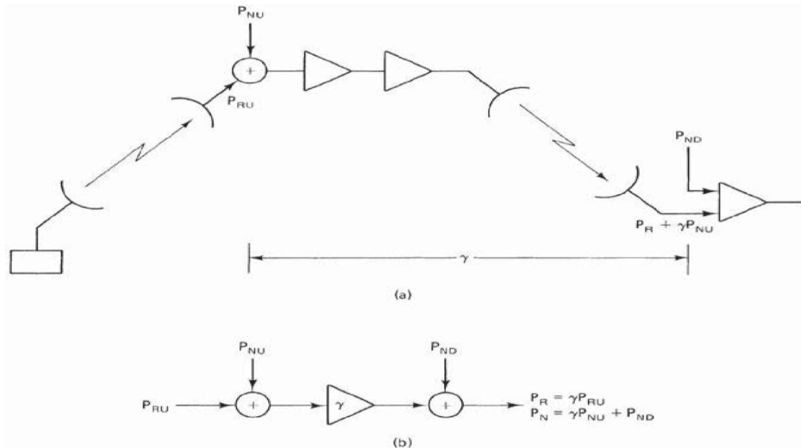
Figure 2.17 (a) Combined uplink and downlink; (b) power flow diagram
