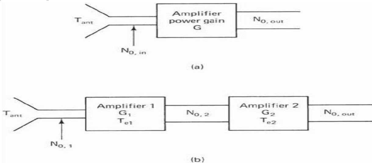
Figure 2.15 LNA Amplifier gain
