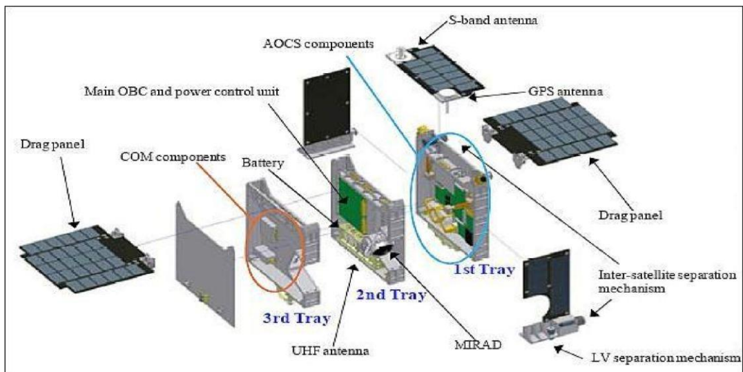
Figure 2.1 (a) Satellite Structure
