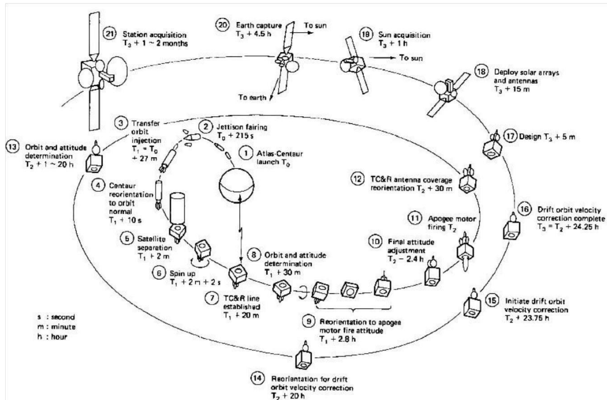
Figure: Launching stages of a GEO (example INTELSAT )
