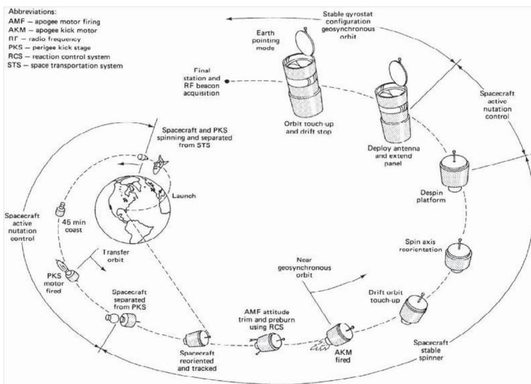
Figure : STS-7/Anik C2 mission scenario. (From Anik C2 Launch Handbook ; courtesy of Telesat, Canada.)
