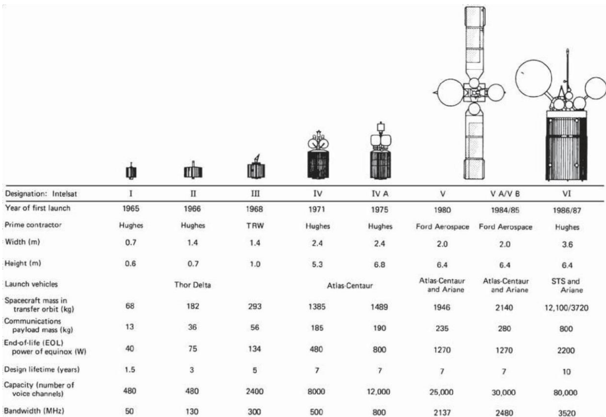
Figure 5.1 INTELSAT Series
