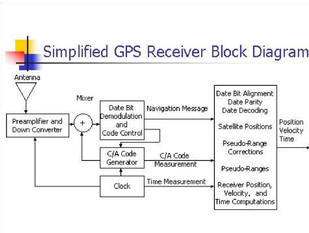
Figure 5.6 GPS Block Diagrams
