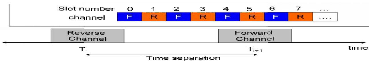
Figure 3. 6 Time Slot
