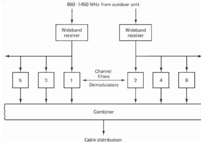
Figure 4.5 One possible arrangement for the indoor unit of a community antenna TV (CATV) system.
