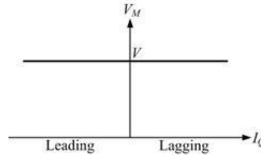
Fig. 2.5: Voltage-current characteristic of an ideal shunt compensator
