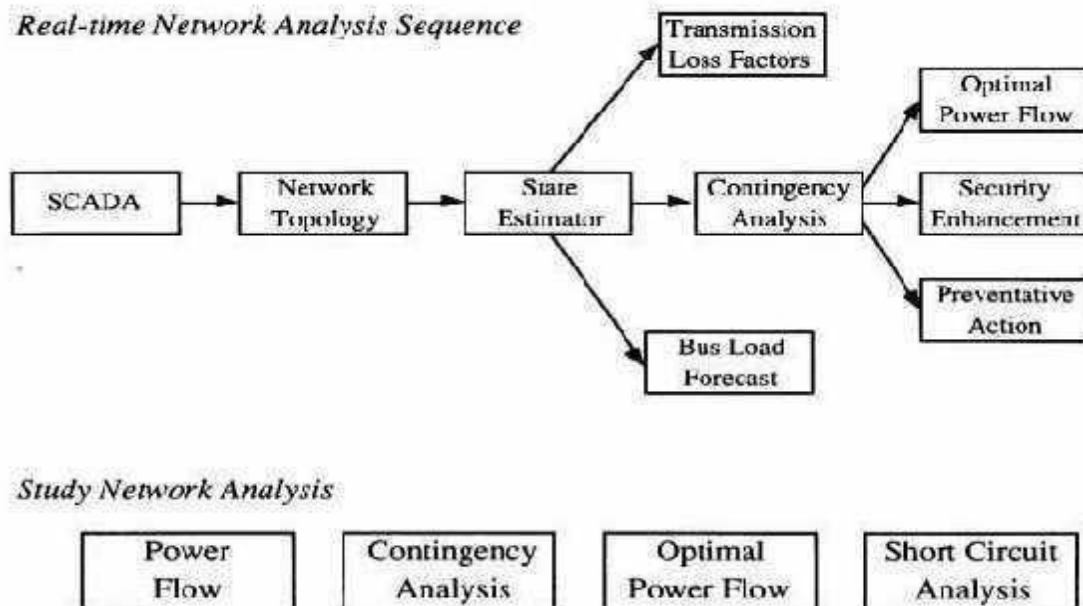
Fig.5:Real time network analysis sequence
