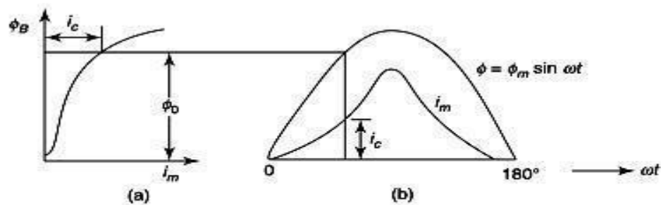
Transformer magnetisation (without hysteresis) (a) Magnetisation curve (b) Flux and magnetisation current waveforms
