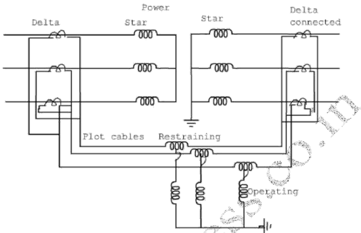
Fig: Differential protection of star-star
