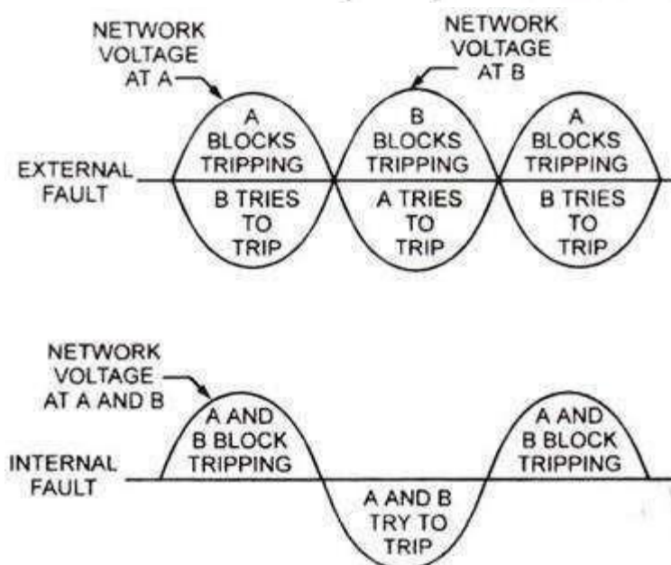
Fig. 5.20. Relations Between Network Output Voltages and Carrier-Current Signals
