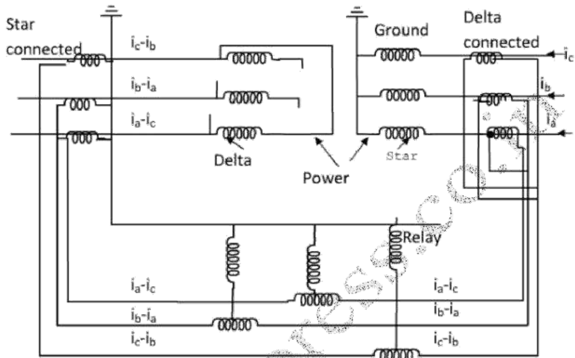
Fig: Differential protection of delta star
