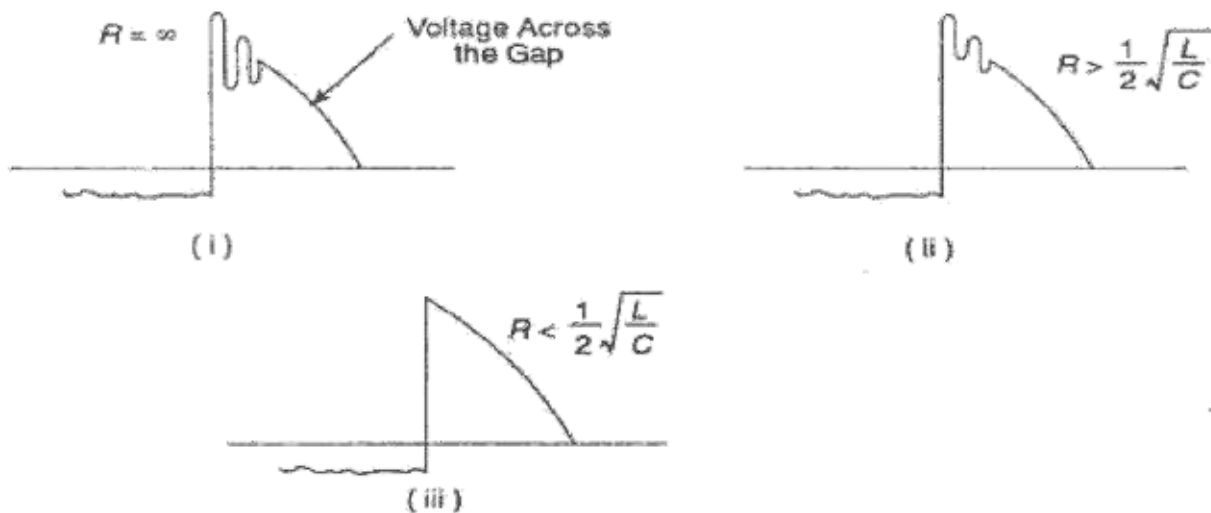
FIGURE 9.9 Transient oscillations for different values of R
