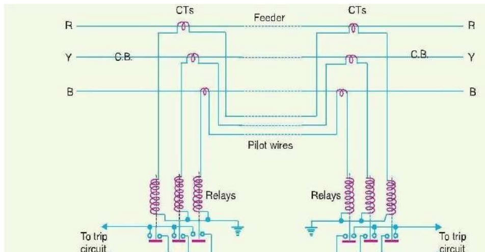
Fig. 23.9 shows the connections of Merz-Price voltage balance scheme for all the three phases of the line.
