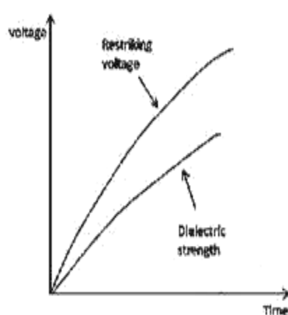
(a) Arc Extinguishes
