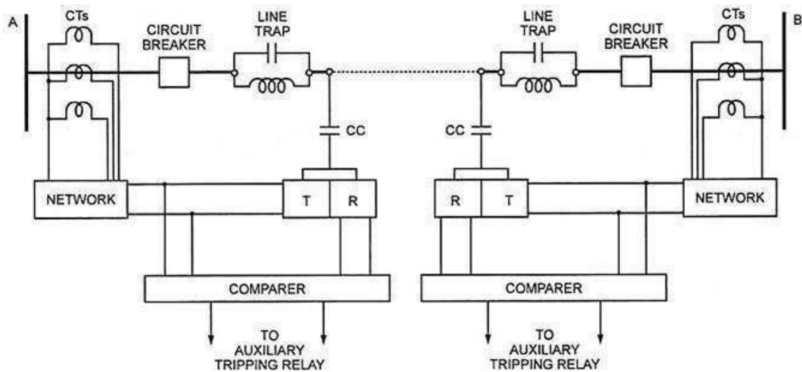
Fig. 5.19. Schematic Representation of Phase-Comparison Carrier Protection
