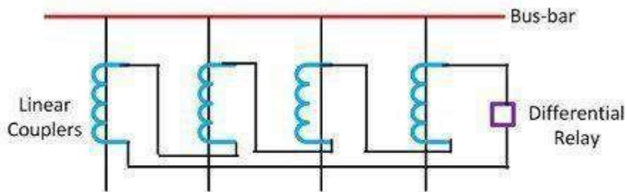
Voltage Differential Relaying For Bus-bar
