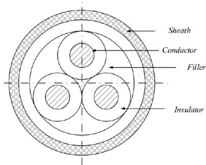
FIG.-7.3 THREE-CORE BELTED TYPE CABLES
