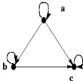
Digraph for Partial Order
