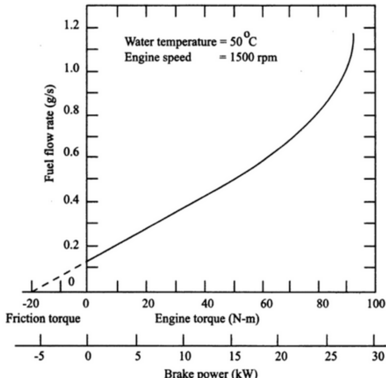
Fig. 9. 8 Willan's line method
