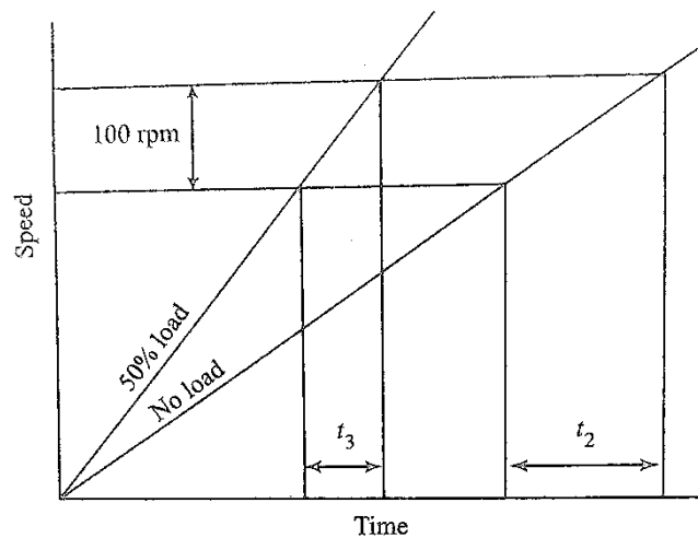
Fig. 9. 9 Graph for Retardation Test
