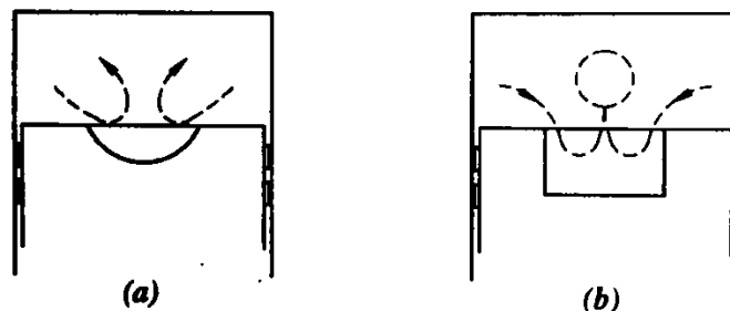
Fig.7. 23 Compression Swirl
