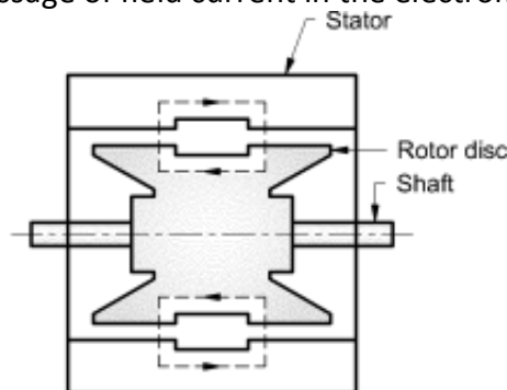
Fig. 9. 6 Eddy current dynamometer
