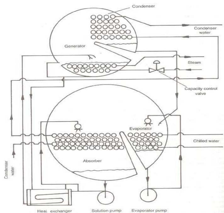
Schematic Diagram of Absorption System of Refrigeration
