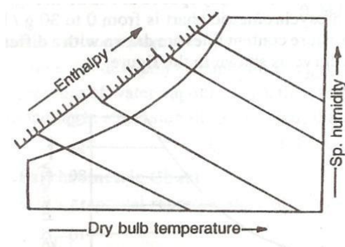
Constant Enthalpy Lines
