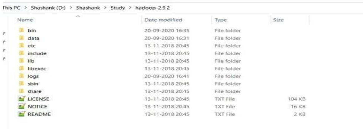
Fig. 4:- Hadoop Directory
