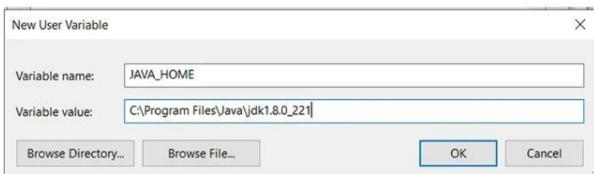
Fig. 8:- Adding JAVA_HOME
