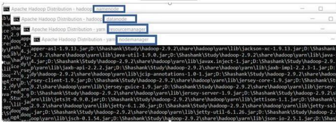
Fig. 17:- Hadoop Daemons
