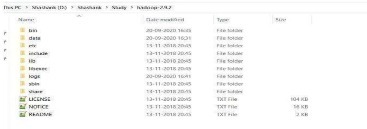
Fig. 4:- Hadoop Directory
