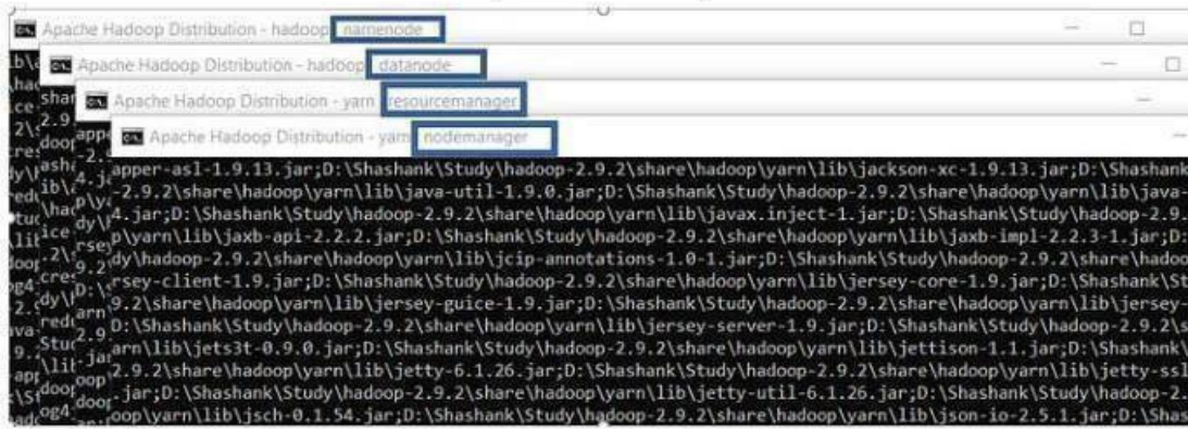
Fig. 17:- Hadoop Deamons
