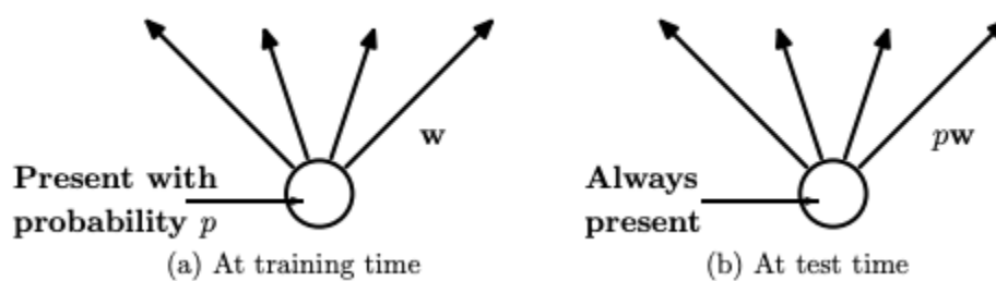
Figure 3: (a) A unit (neuron) during training is present with a probability p and is connected to the next layer with weights ' w '; (b) A unit during inference/prediction is always present and is connected to the next layer with weights, ' pw '
