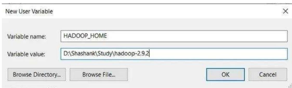
Fig.10:- Adding HADOOP_HOME
