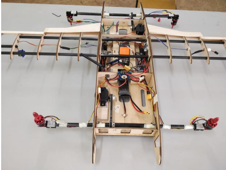
Skeletal frame with all electronic components
